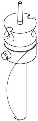
PICK-UP NOZZLE (ID= \phi 0.5, OD= \phi 0.8) SONY SMT
