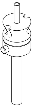
PICK-UP NOZZLE (ID= \phi 1.2, OD= \phi 1.6) SONY SMT
