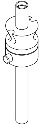
PICK-UP NOZZLE (ID= \phi 2.5, OD= \phi 3.0) SONY SMT
